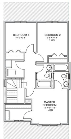
Upper Level 699 sq. ft.
