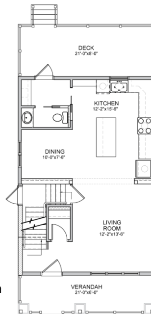
Main Floor 640 sq. ft.
