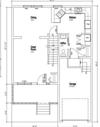
Two-storey (main floor)
